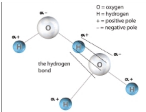
A water molecule is the smallest magnet.
