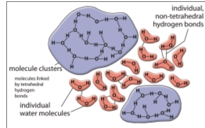
By forming so-called "molecule clusters", water develops a "memory".
