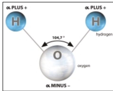
The chemical structure of a water molecule.
